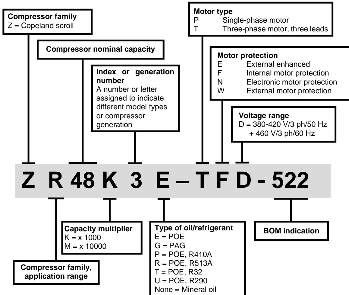
Figure 1: Example of nomenclature for a standard scroll compressor, ZR range
